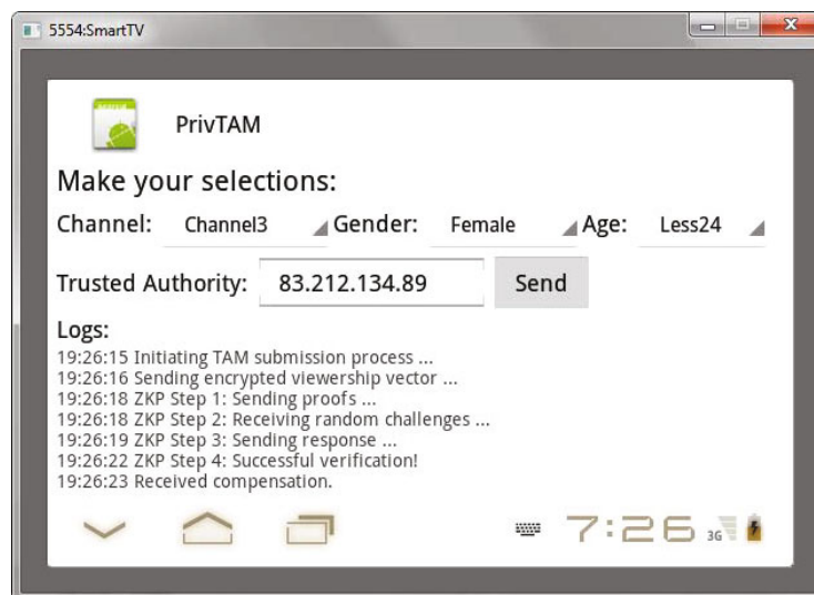
Fig. 4. A snapshot of the TVAgent s
